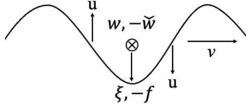
FIG. 1. Wave variables at their maximal positions for a plane wave propagating toward the right with speed v . When displacement \xi is downward, the force density f is upward, the angular velocity w of the medium is into the page, and the wave velocity rotation rate \tilde{w} relative to the medium is opposite to w .
